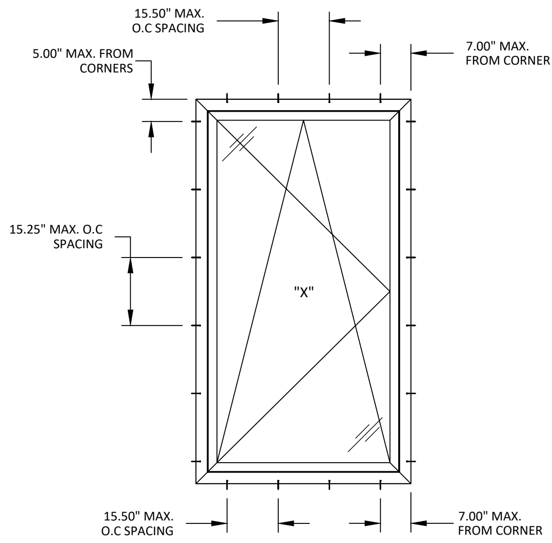
ANCHOR LAYOUT THROUGH FRAME INSTALLATION
