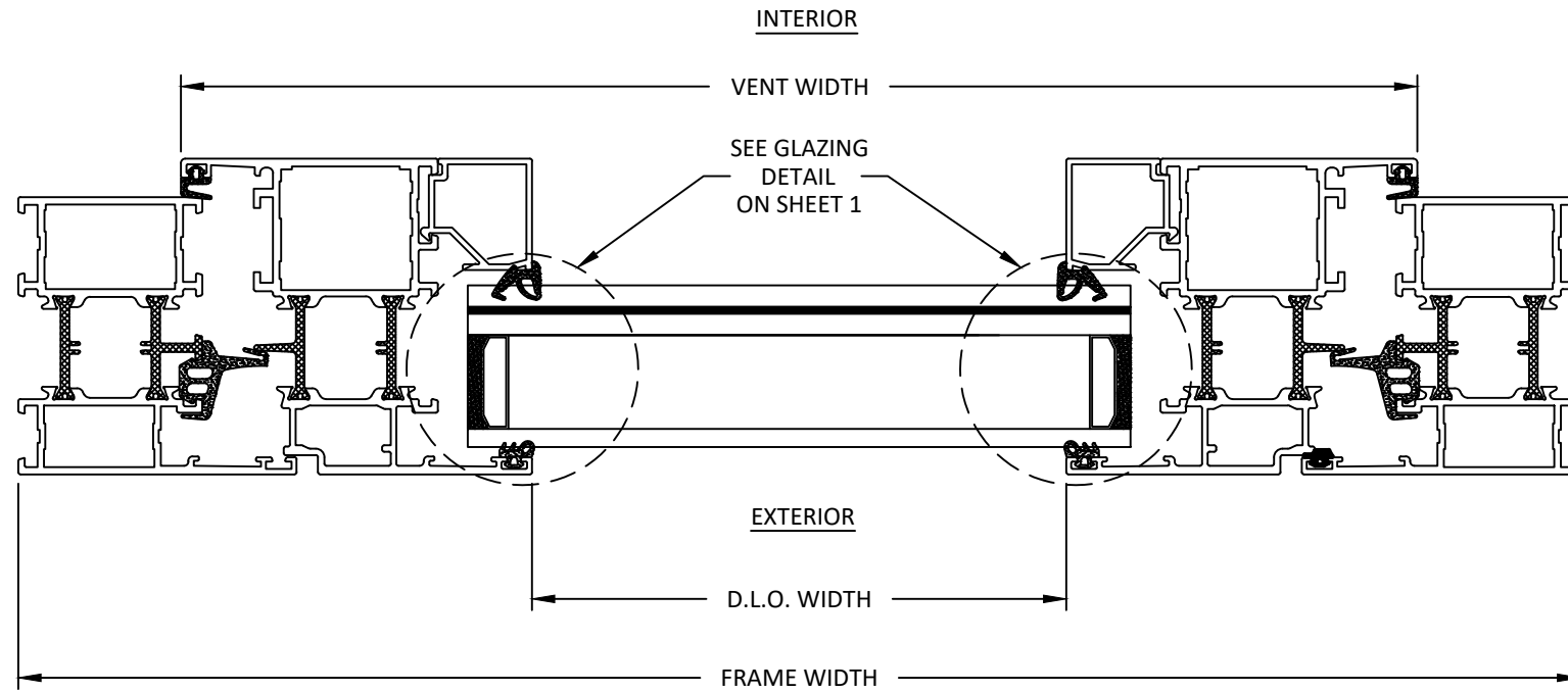
A HORIZONTAL SECTION 6 IMPERIAL TILT & TURN WINDOW
