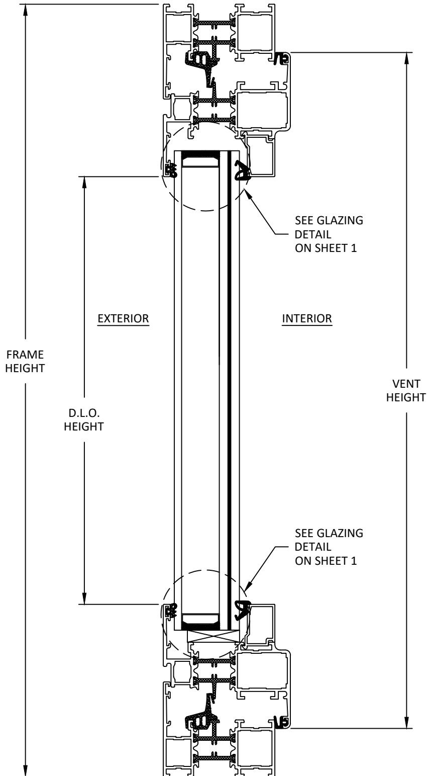
A 5 VERTICAL SECTION IMPERIAL TILT & TURN WINDOW
