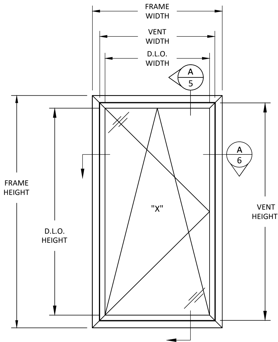
ELEVATION X CONFIGURATION
