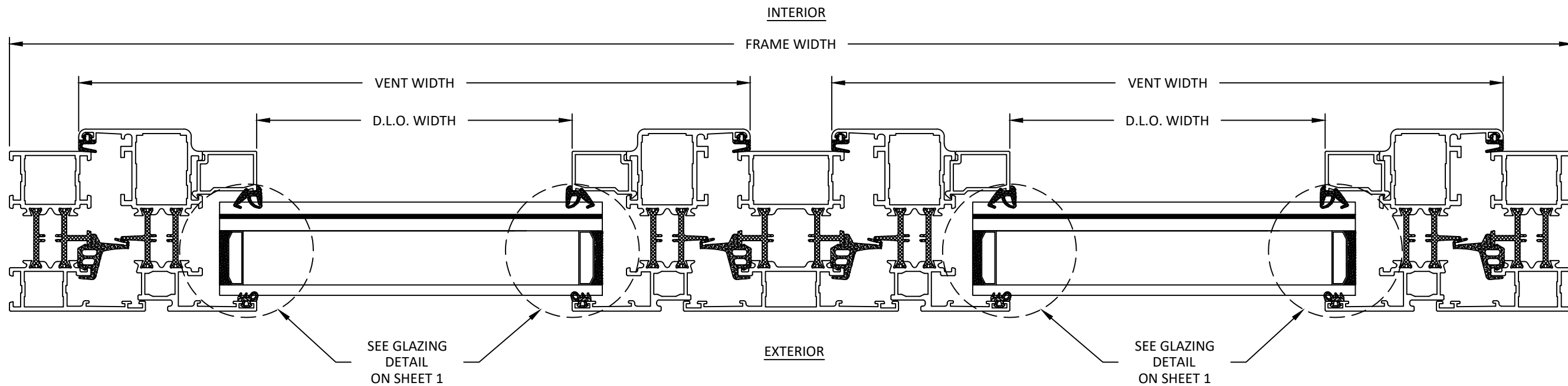
B6 HORIZONTAL SECTION IMPERIAL TILT & TURN WINDOW
