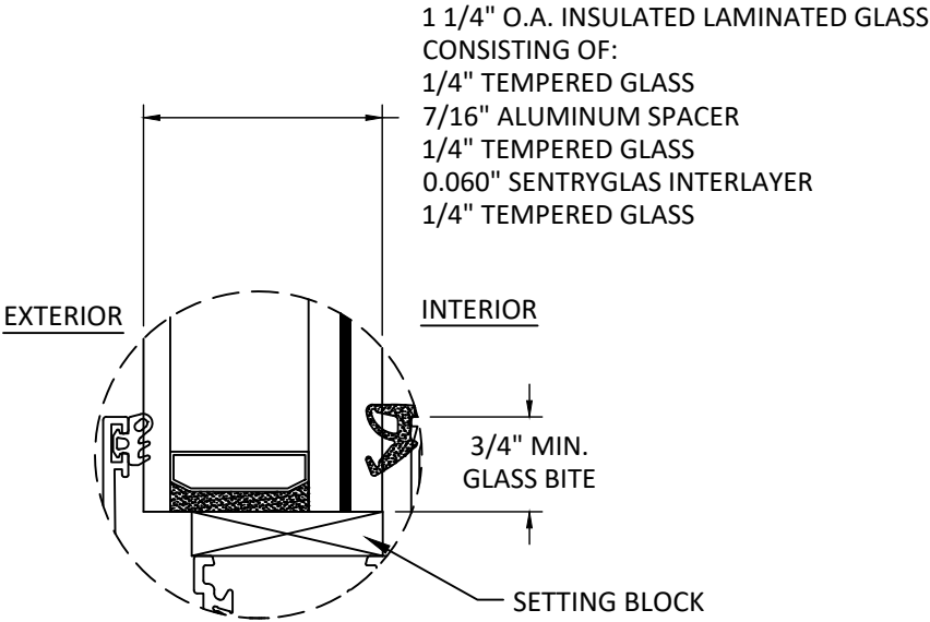
GLAZING DETAIL 1
