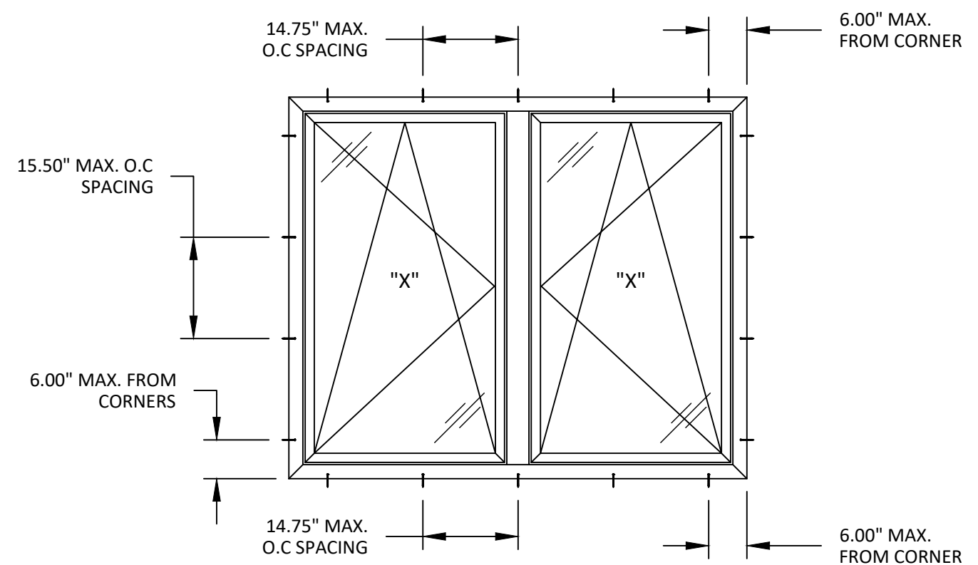
ANCHOR LAYOUT THROUGH FRAME INSTALLATION
